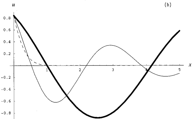
FIG. 5. (a) |u_{\infty}| vs x for dry air with \mu = 1.7 \times 10^{-5} Pa sec, \rho_0 = 1.293 kg/m 3 , and \omega = 5.0 kHz. Bold line: c = 361.0 m/sec; solid line: c = 331.0 m/sec; and broken line: c = 301.0 m/sec. (b) u vs x (ND) for t = 0.1 and \omega = 10.0 . Bold line: c = 10.0 ; solid line: c = 5.0 ; and broken line: c = 0.05 .
